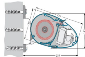
Wandmontage
