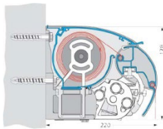
Wandmontage
