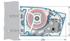
Wandmontage
