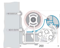
Wandmontage
